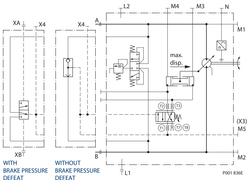
Circuit Diagram – Motor with Pressure Compensator Control TA**
