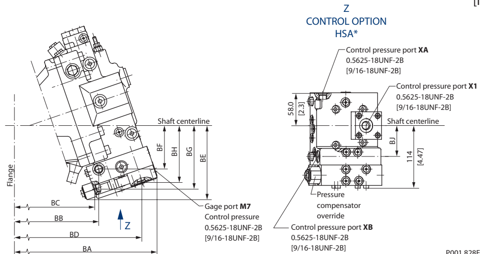
Control Option HSA* for 51
