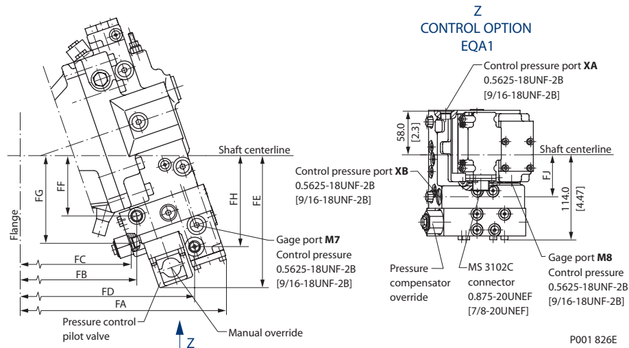
Control Options EPA1, EQA1 for 51
