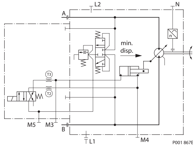
Circuit Diagram–Motor with Electrohydraulic Two-Position Control F1B1,F2B1,
