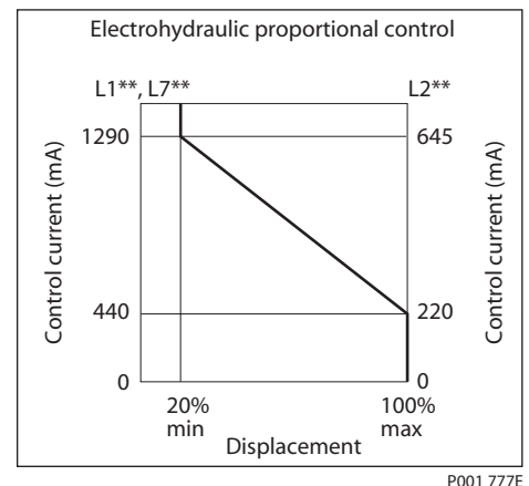
Control Operation L1**, L2**, L7**
