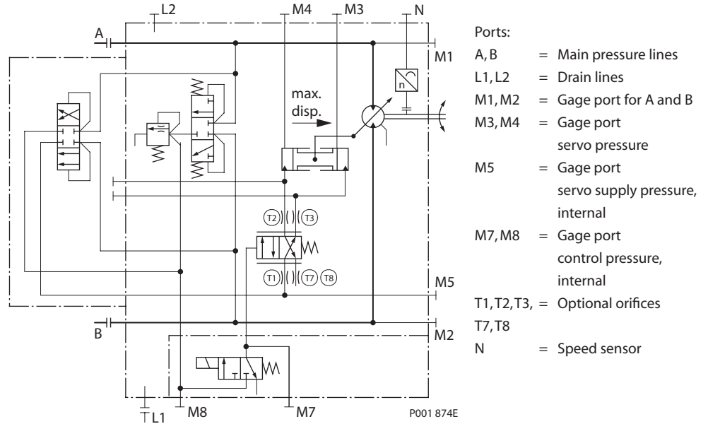
Circuit Diagram – Motor with Electrohydraulic Two-Position Control F1A5, F2A5
