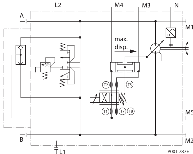
Circuit Diagram – Motor with Electrohydraulic Proportional Control L1B1, L2B1, L7B1
